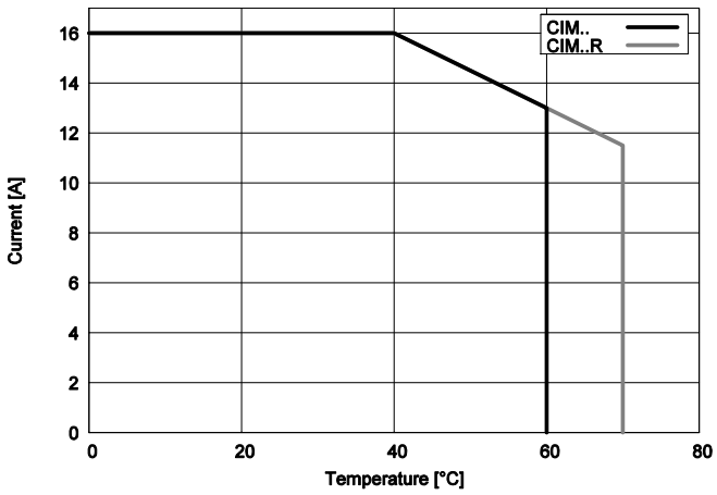
CIM2, CIM2R - Output current
