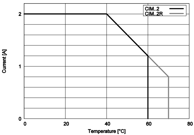
CIM22, CIM22R - Output current
