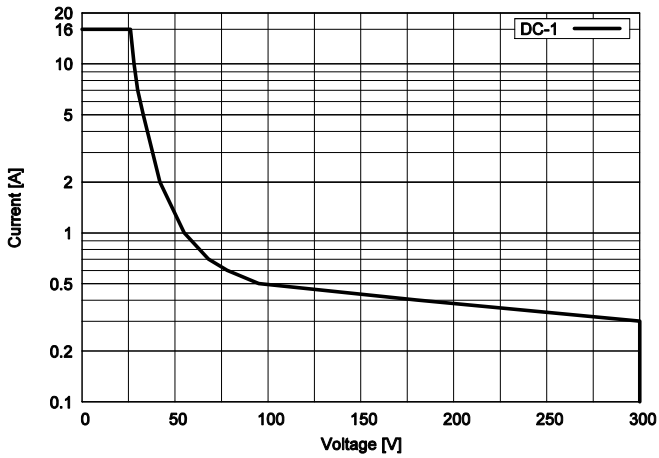
CIM2, CIM2R - Breaking capacity
