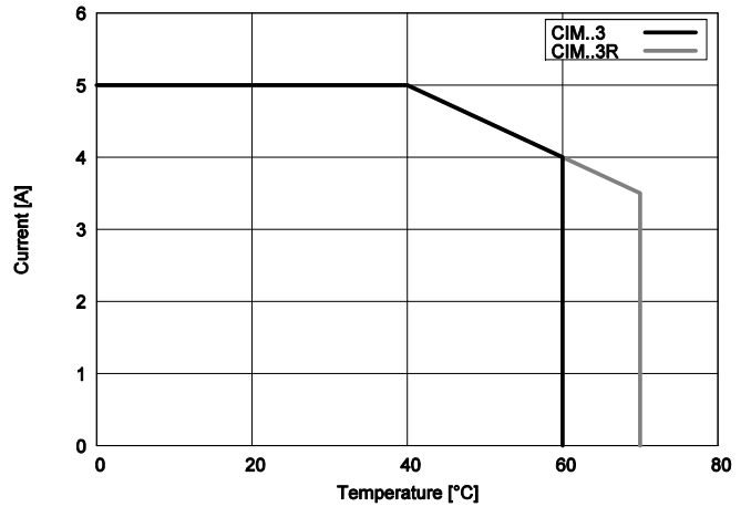
CIM23, CIM23R - Output current
