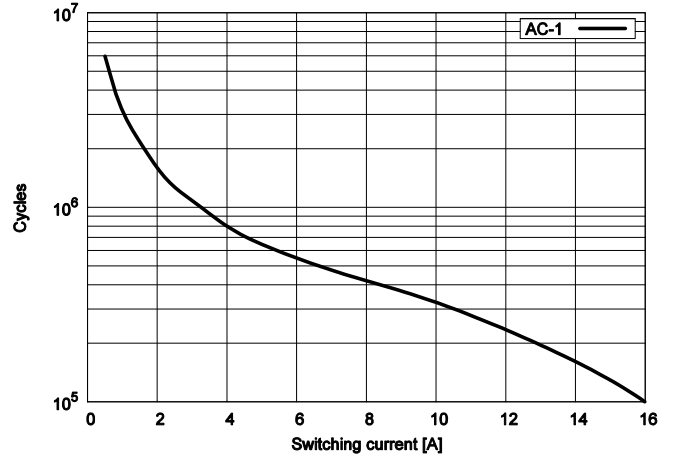
CIM2, CIM2R - Electrical endurance
